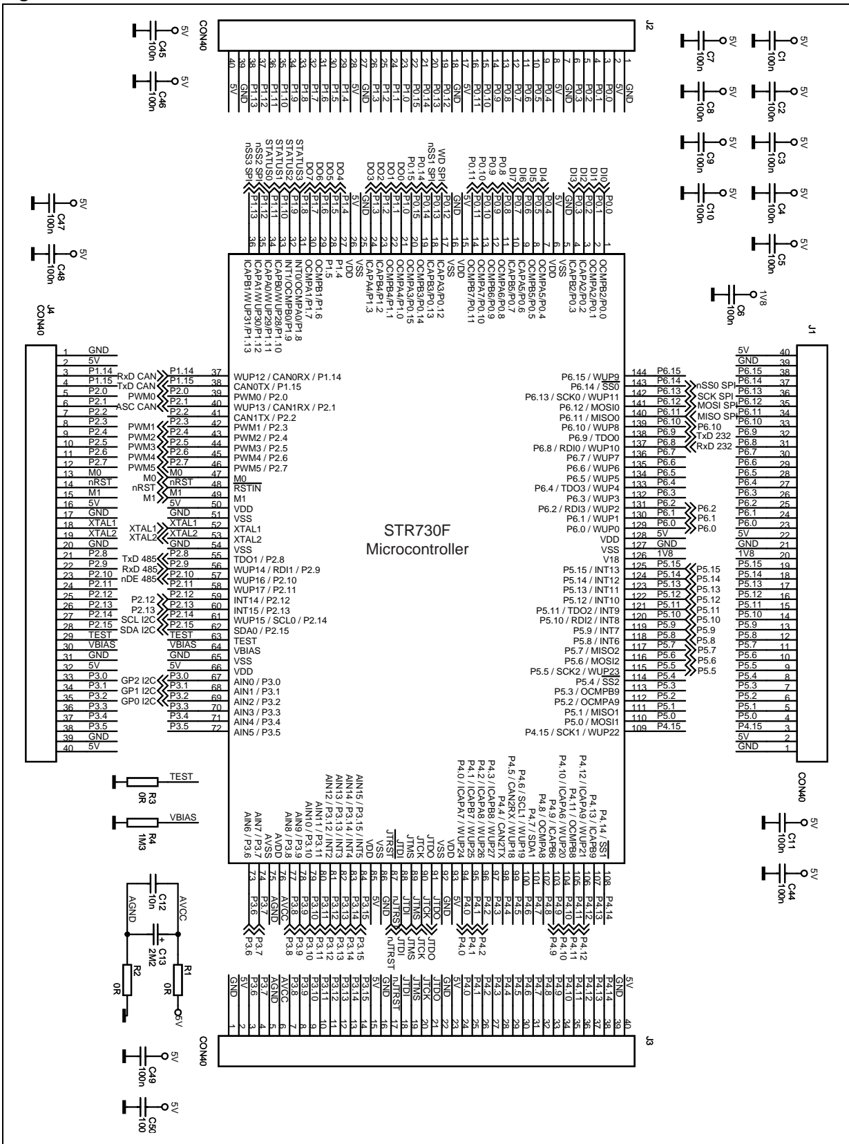
Figure 27. MCU schematic
